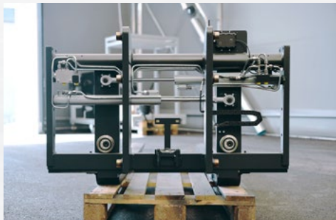
C35 with SmartFork® SideCam
