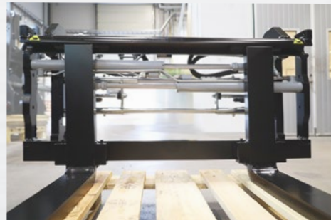
C25 with QQT 300i (automatic quick coupler)
